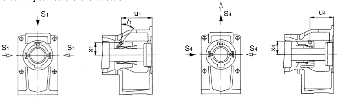
P02 with flushing ring
