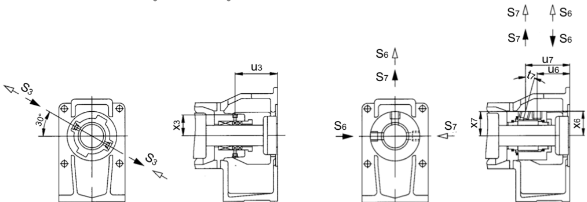
P04 with external sealing chamber ring
