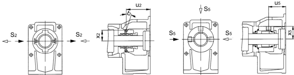
P03 with internal sealing chamber ring
